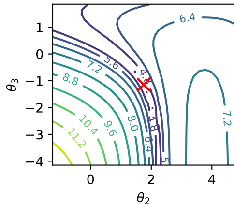
Fixed param: \theta_1
