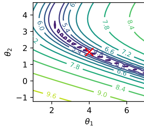
Fixed param: \theta_3
