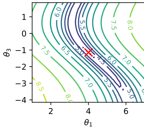
Fixed param: \theta_2
