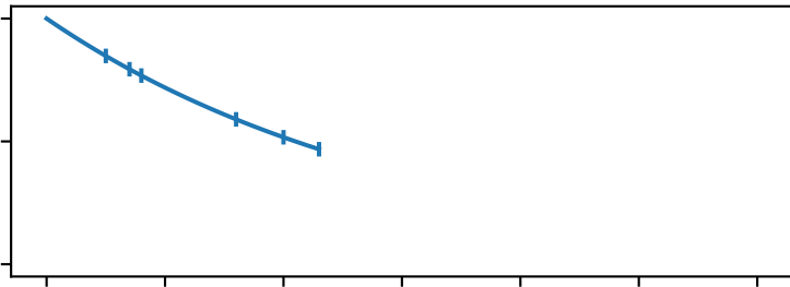
True model
